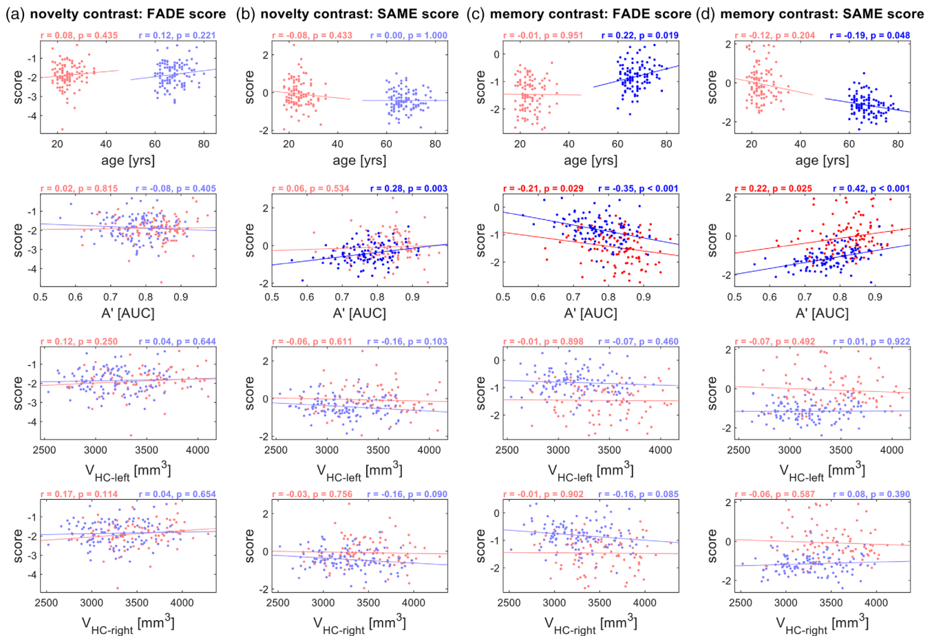
FIGURE 4 Correlations with independent variables, separated by age group. Results from correlation analyses of FADE-classic and FADE-SAME scores with age, memory performance ( A' ) and hippocampal volumes ( V_{HC} ). Correlations are reported separately for (a) the classic FADE score computed from the novelty contrast, (b) the FADE-SAME score computed from the novelty contrast, (c) the classic FADE score computed from the memory contrast, and (d) the FADE-SAME score computed from the memory contrast. Young subjects are depicted in red, and older subjects are depicted in blue. Significant correlation coefficients are highlighted
